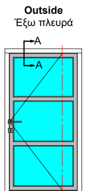
FRONT VIEW Όψη
