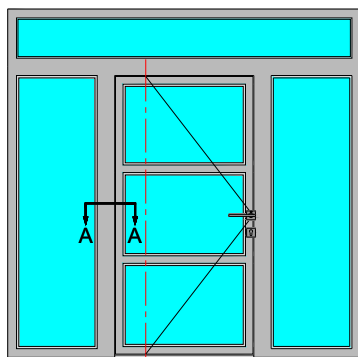
FRONT VIEW ΟΨΗ
