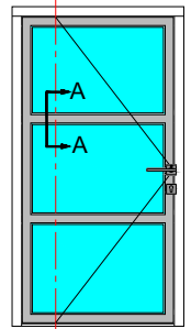
FRONT VIEW Όψη
