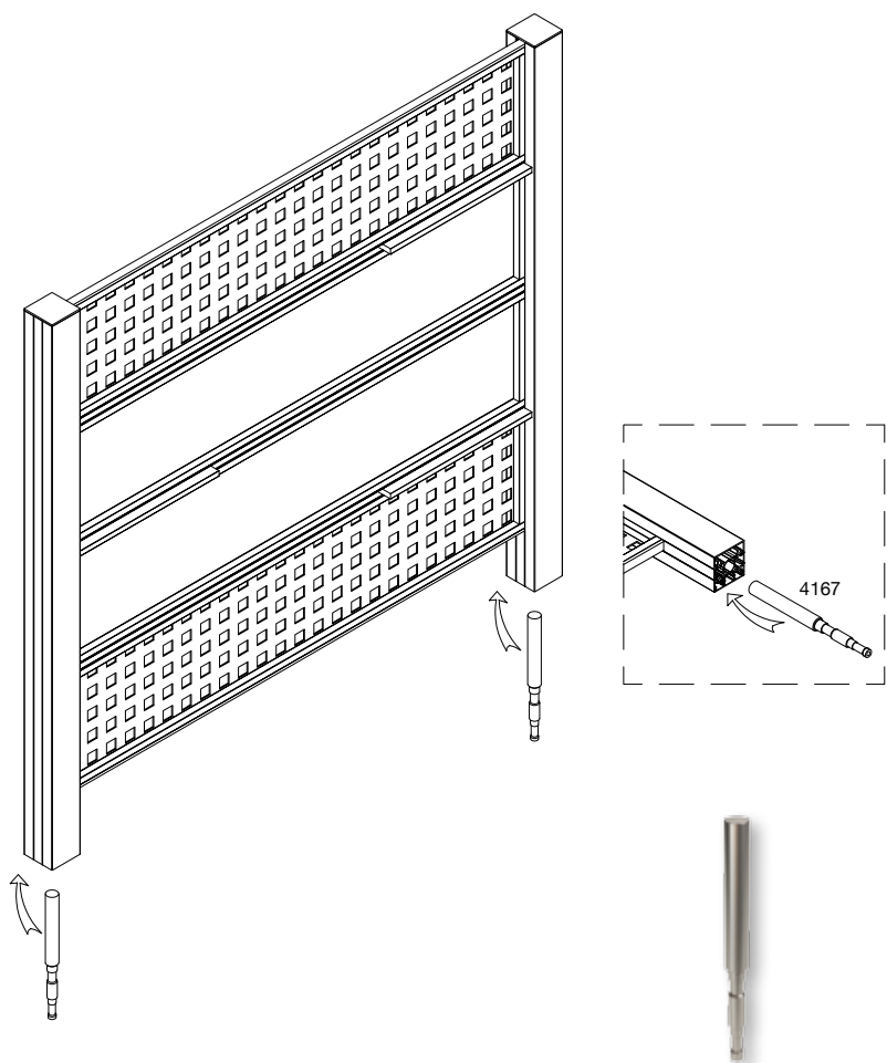
Infloor support for Ø42 columns Code 4167
