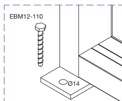
Concrete Screw Ø12-110
