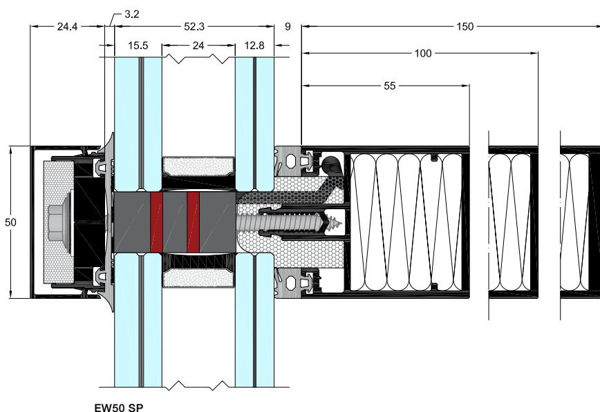
EW50 SP
