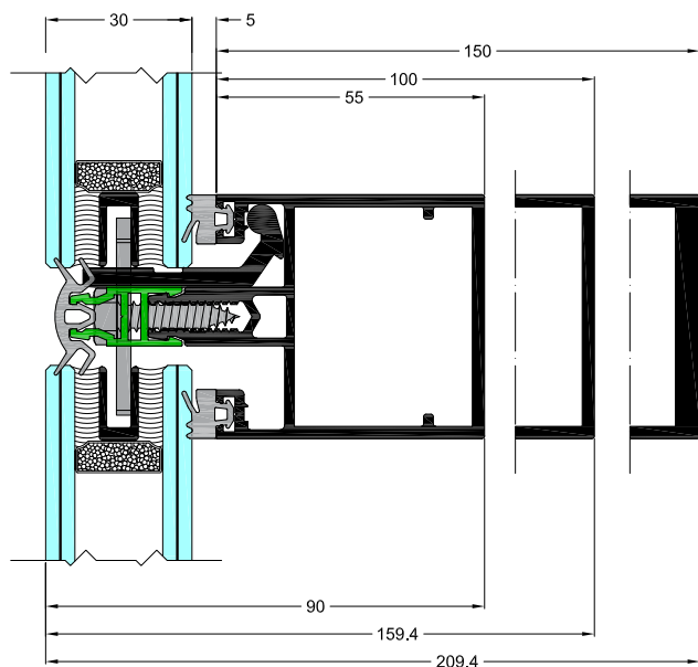
Structural EW50
