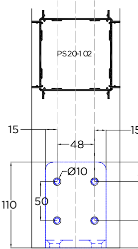
POST HOLES DRILLING FOR FIXING FOOTPLATE
