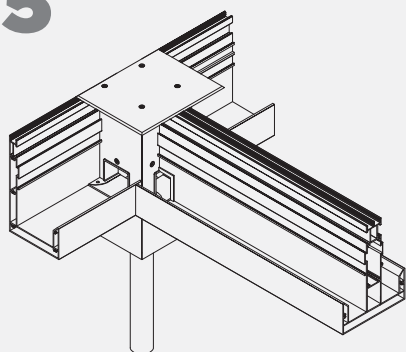
POST-TAY CONNECTION
