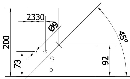
APS20-1218 HOLE CUT
