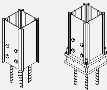
STANDARD FOOTPLATE (APS20-1211)
