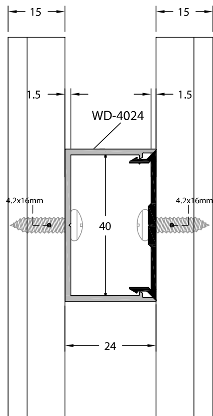
SIDE VIEW B-B
