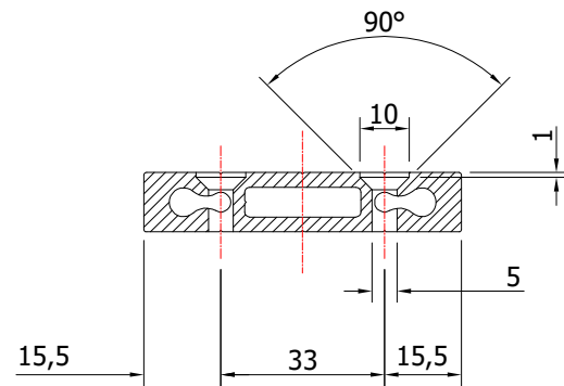
Section A-A (DOUBLE HOLE)
