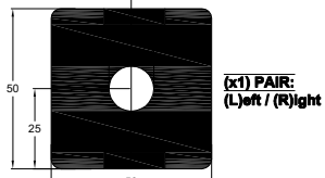
ALUMINIUM ROZETTES:
