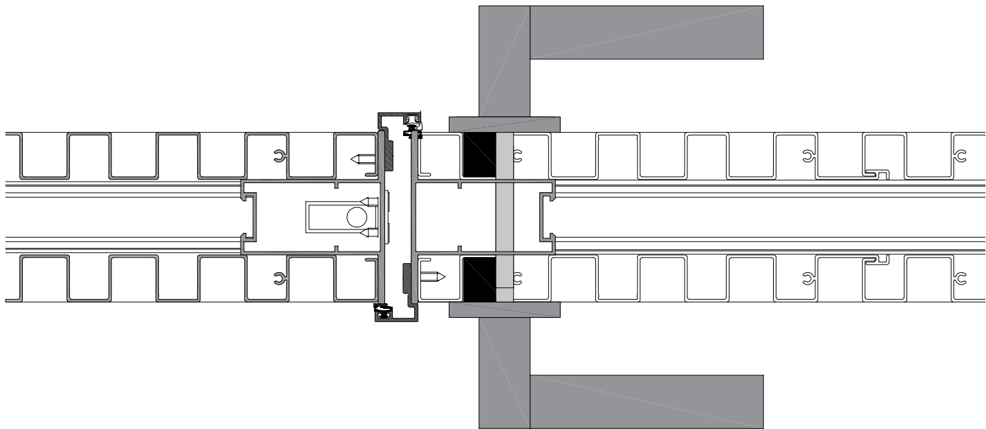
Detail View-A
