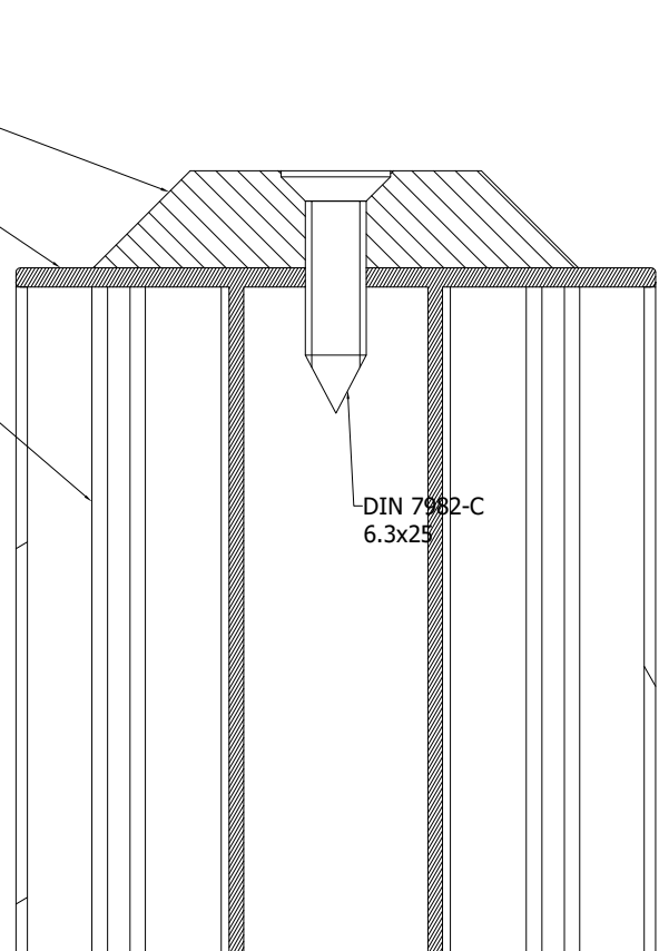
Detail View (Top Connector) WD2040 Vertical
