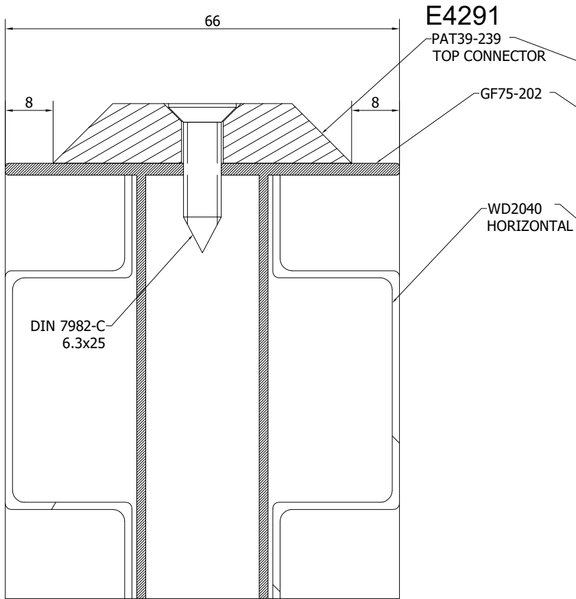
Detail View (Top Connector) WD2040 Horizontal
